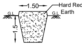
Trial Pit
