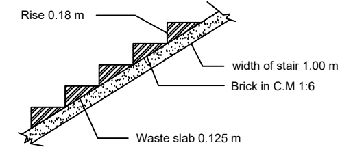
Stair Details
