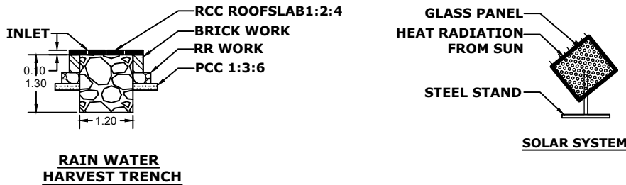
RAIN WATER HARVEST TRENCH
