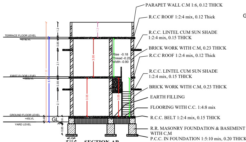
SECTION-AB SCALE- 1:100
