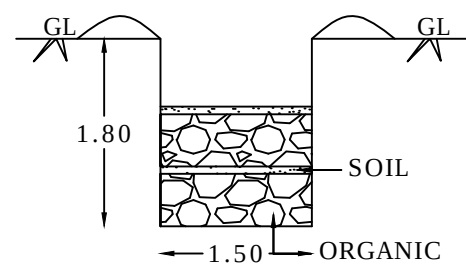
COMPOST PIT
