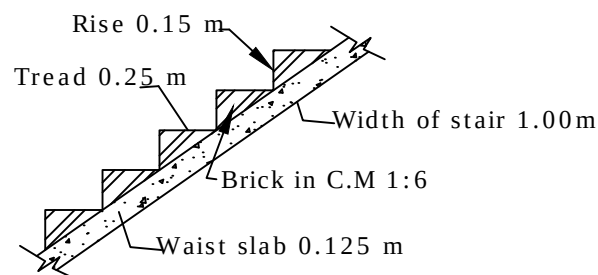
STAIR DETAILS
