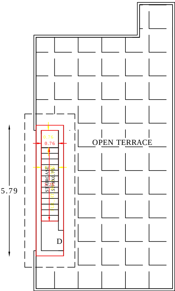
HEAD ROOM PLAN
