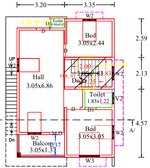
EXISTING & EXTENSION FIRST FLOOR PLAN
