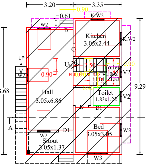
EXISTING & EXTENSION GROUND FLOOR PLAN
