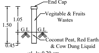
PIPE COMPOSTER
