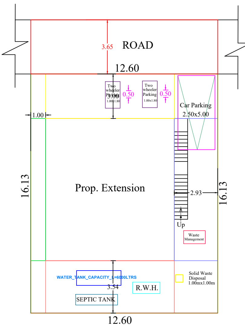
SITE PLAN
