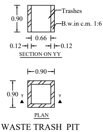
WASTE TRASH PIT
