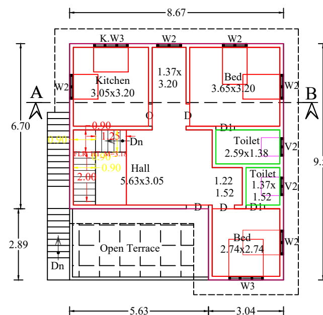
EXTENSION FIRST FLOOR PLAN
