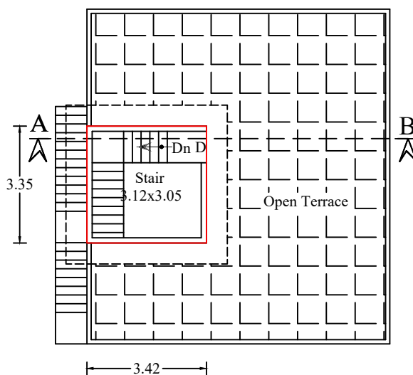
HEAD ROOM PLAN
