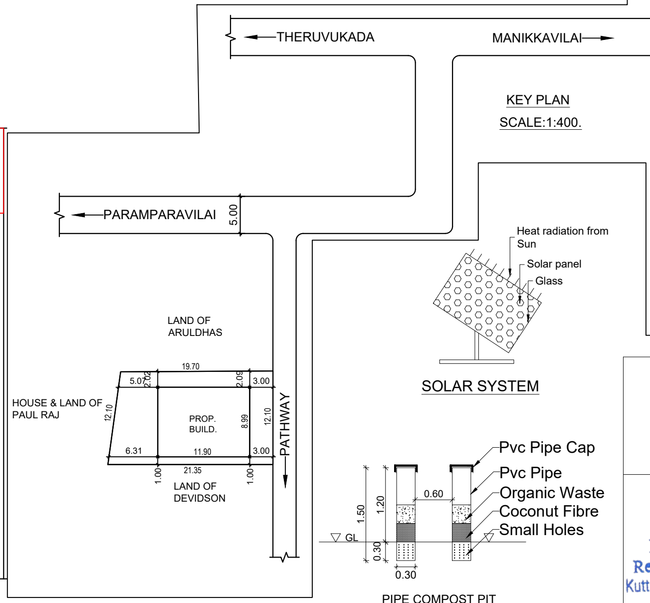
PIPE COMPOST PIT
