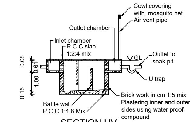
SECTION UV
