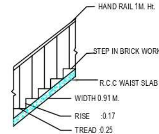
STAIR DETAIL
