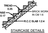
STAIRCASE DETAILS
