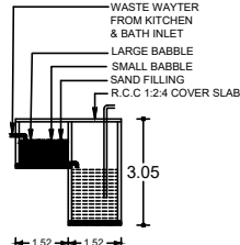
RECYCLING OF WASTE WATER TANK
