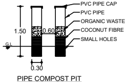
PIPE COMPOST PIT
