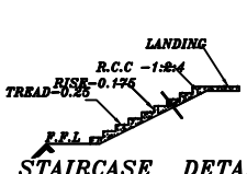
STAIRCASE DETAIL
