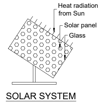
SOLAR SYSTEM
