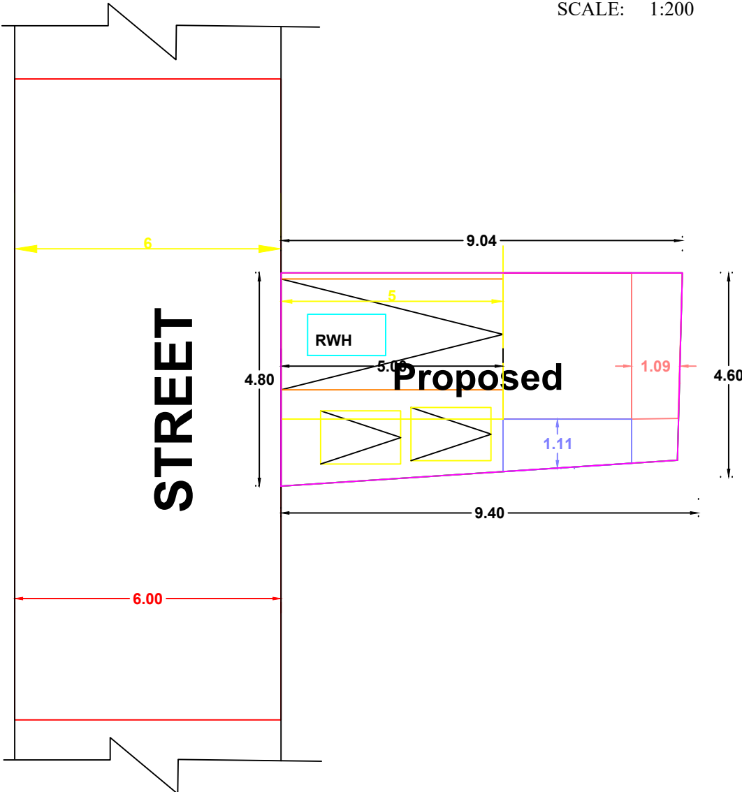
DETAILS OF RAIN WATER HARVESTING
