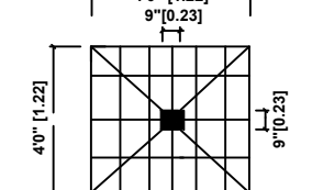
PLAN COLUMN SIZE = 0'9" X 0'9"
