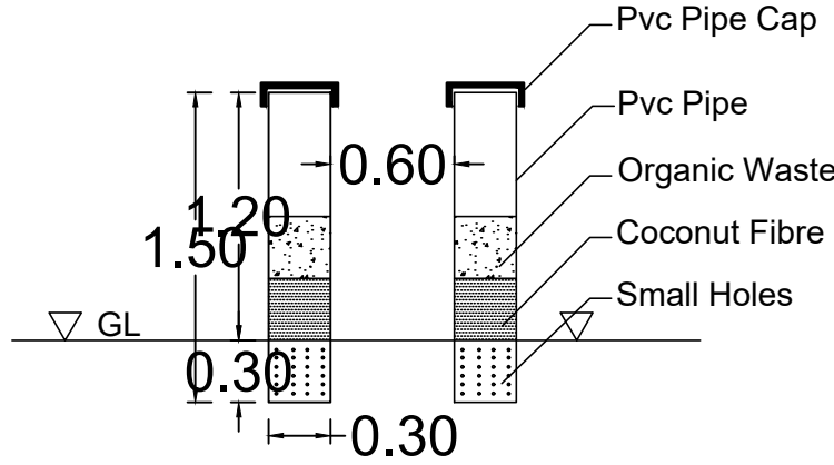
PIPE COMPOST PIT
