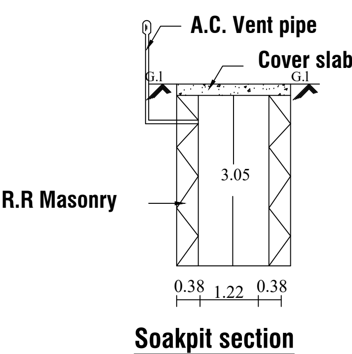
Soakpit section
