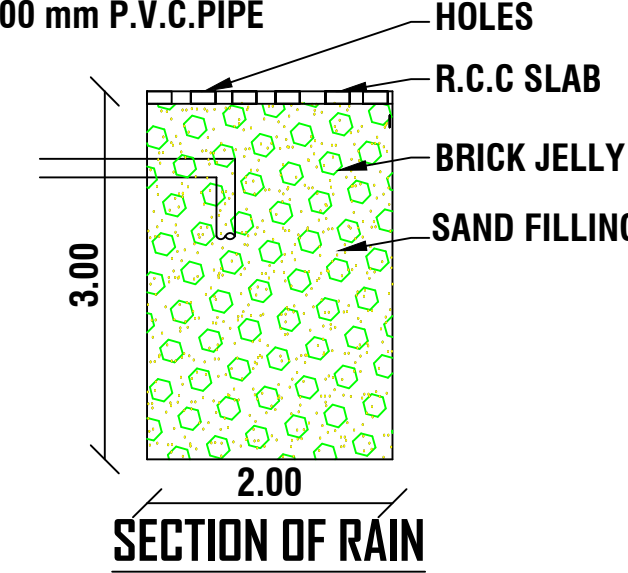
SECTION OF RAIN
