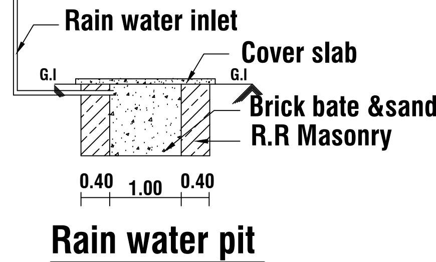
Rain water pit
