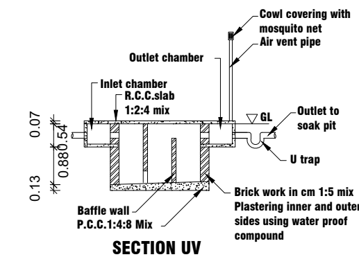
SECTION UV
