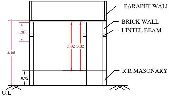
SECTION AT X-X'
