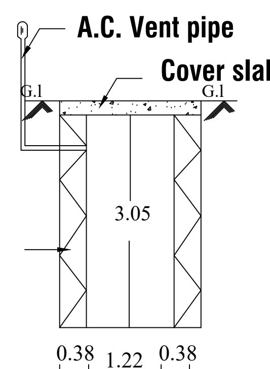
Soakpit section
