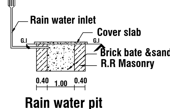
Rain water pit
