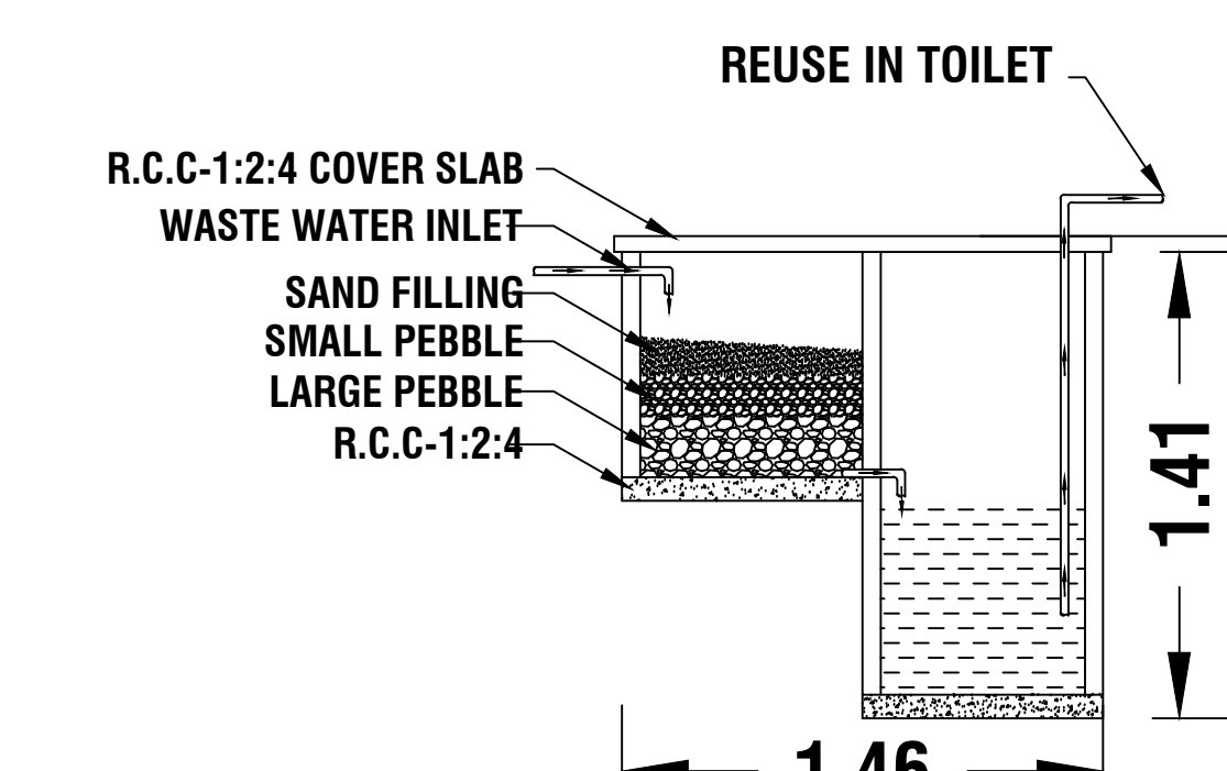
RECYCLING OF WASTE WATER
