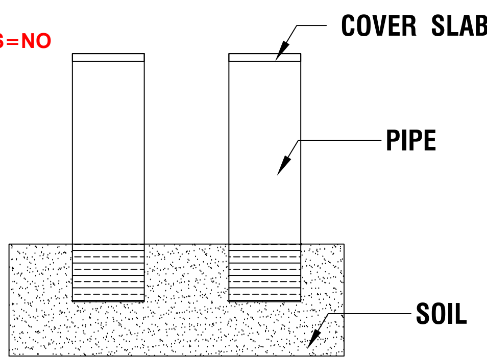
PIPE COMPOSTING
