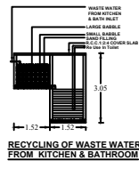
RECYCLING OF WASTE WATER FROM KITCHEN & BATHROOM
