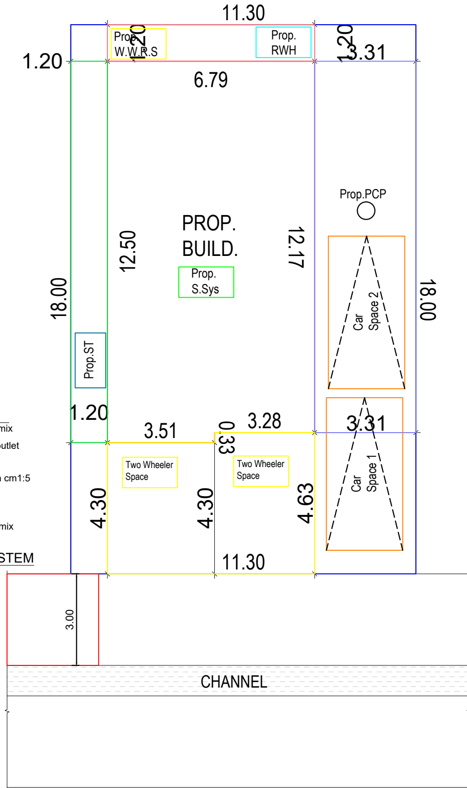
SITE PLAN
