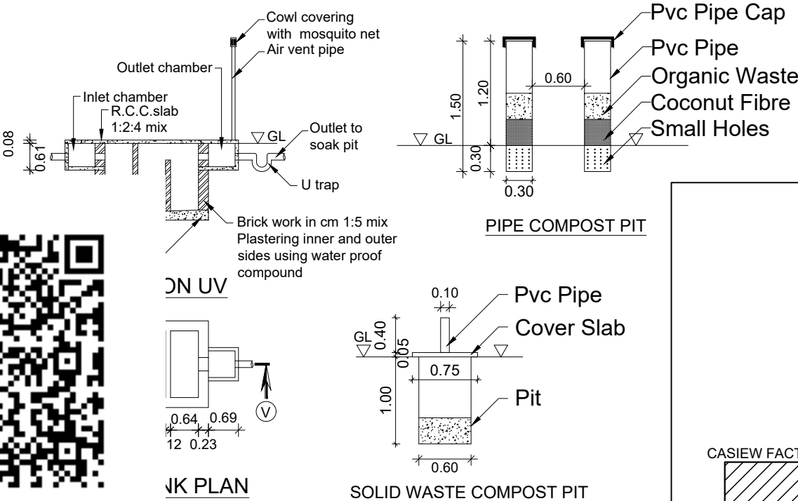
SOLID WASTE COMPOST PIT
