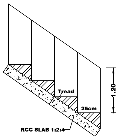
STAIR DETAILS
