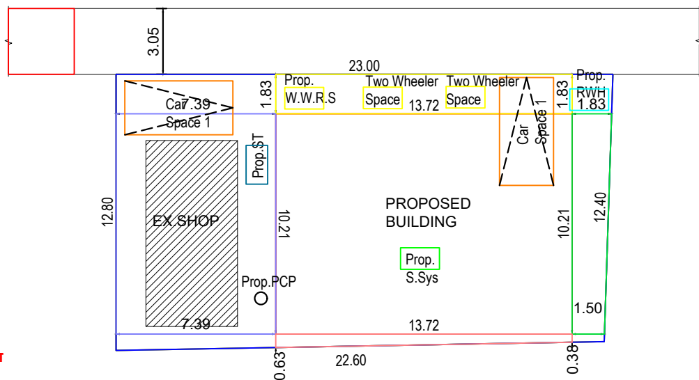
SITE PLAN
