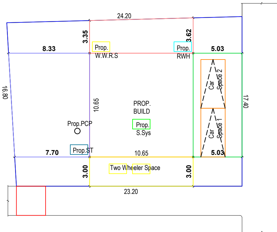
SITE PLAN
