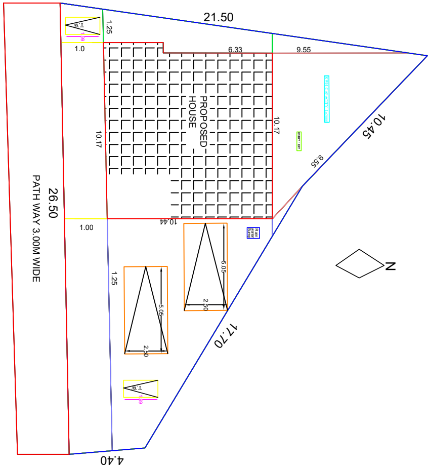
SITE PLAN
