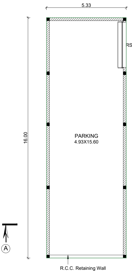
CELLAR FLOOR PLAN (PARKING)
