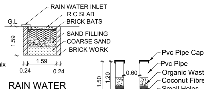
RAIN WATER HARVESTING PIT
