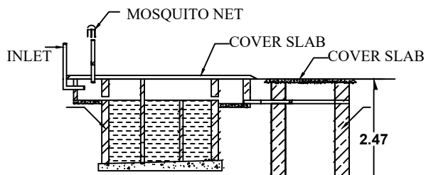
SEPTIC TANK
