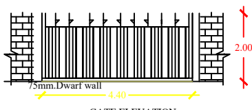
GATE ELEVATION
