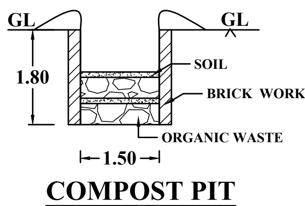
COMPOST PIT
