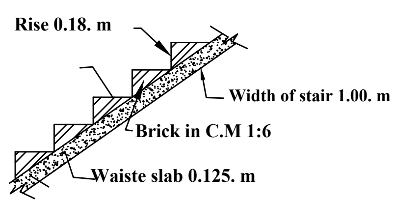
Stair Details
