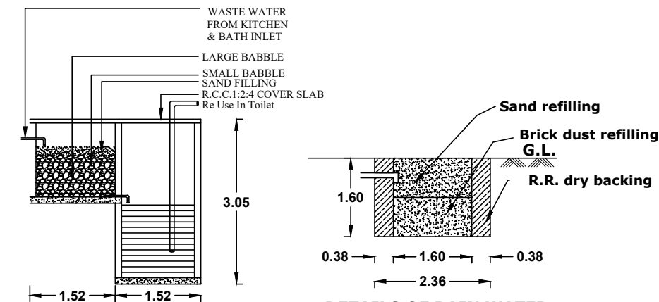
DETAILS OF RAIN WATER HARVESTING
