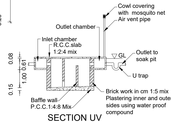
SECTION UV
