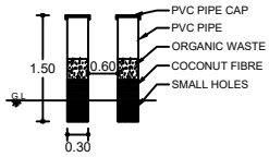
PIPE COMPOST PIT
