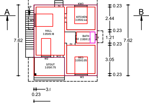
GROUND
