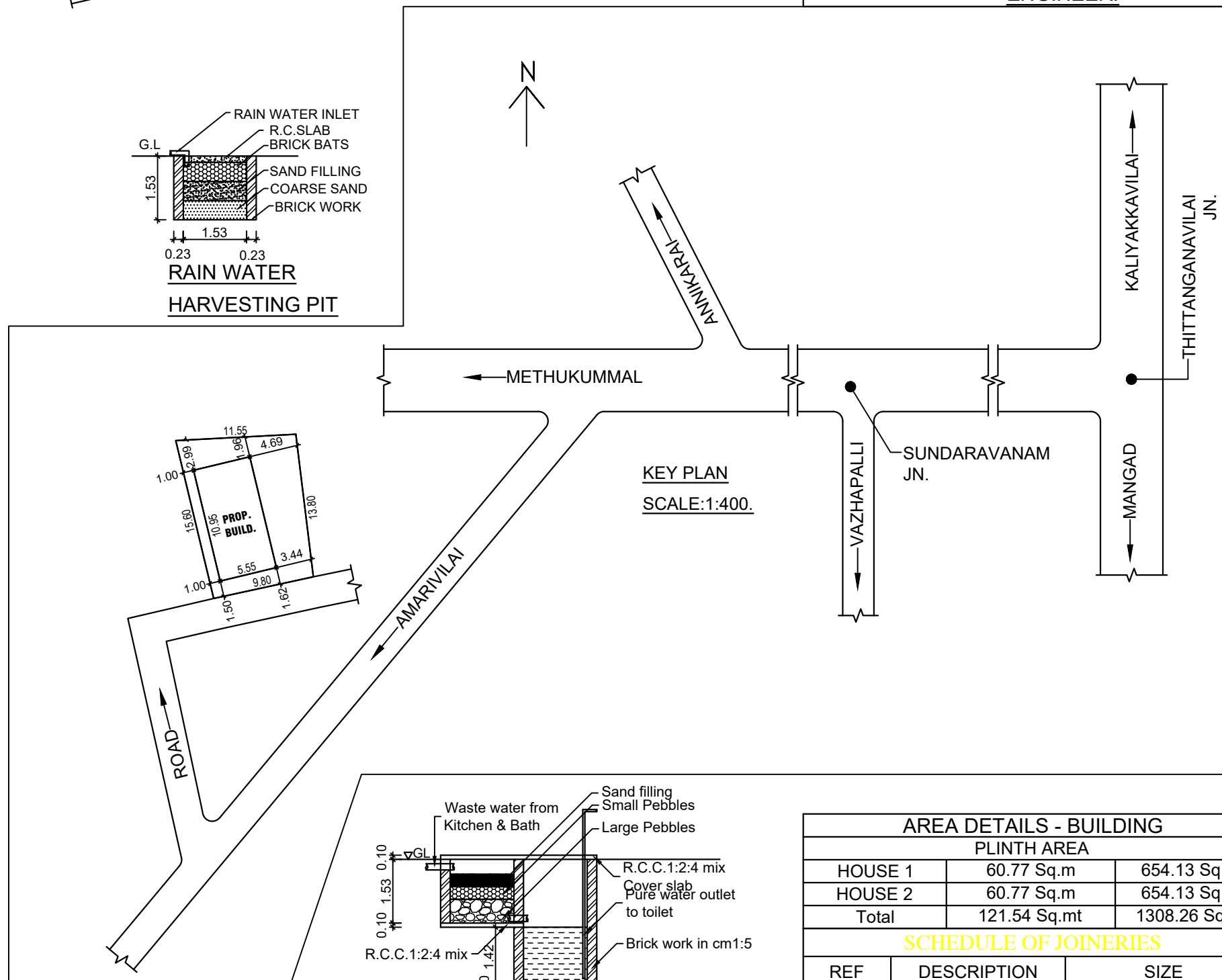
SITE PLAN
