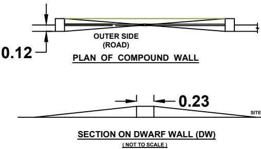
SECTION ON DWARF WALL (DW)
