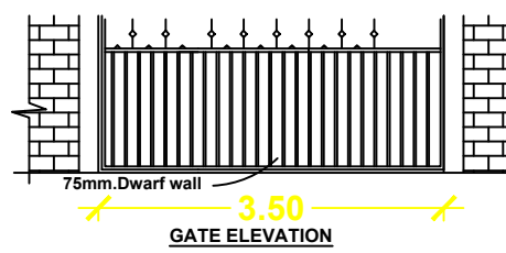
GATE ELEVATION
