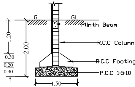
SECTION AT X-X'
