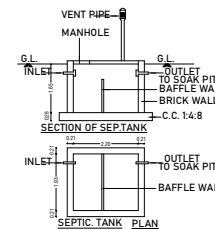
SECTION OF SEPT. TANK
