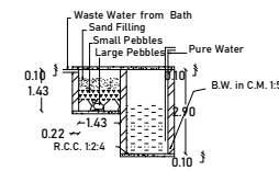
WASTE WATER RECYCLING SYSTEM
