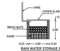
RAIN WATER STORAGE PIT
