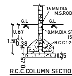
R.C.C. COLUMN SECTION
