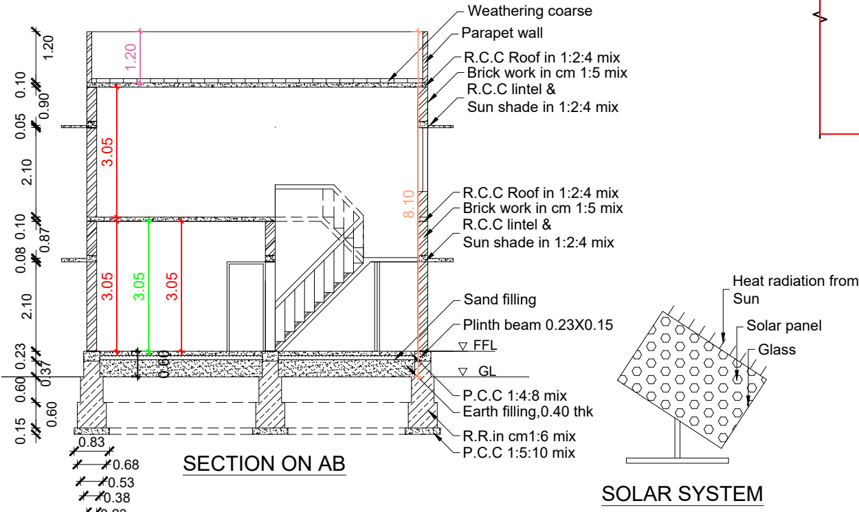
SOLAR SYSTEM
