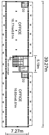
SECOND FLOOR PLAN
