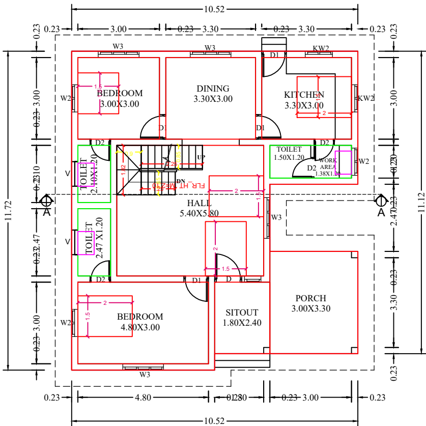
GROUND FLOOR PLAN AREA =112.16 Sq.M (1206.84 Sq.ft) SCALE- 1:100
