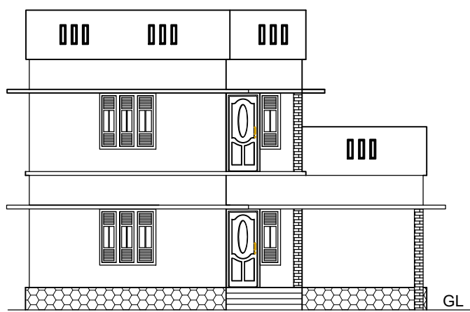
ELEVATION SCALE- 1:100
