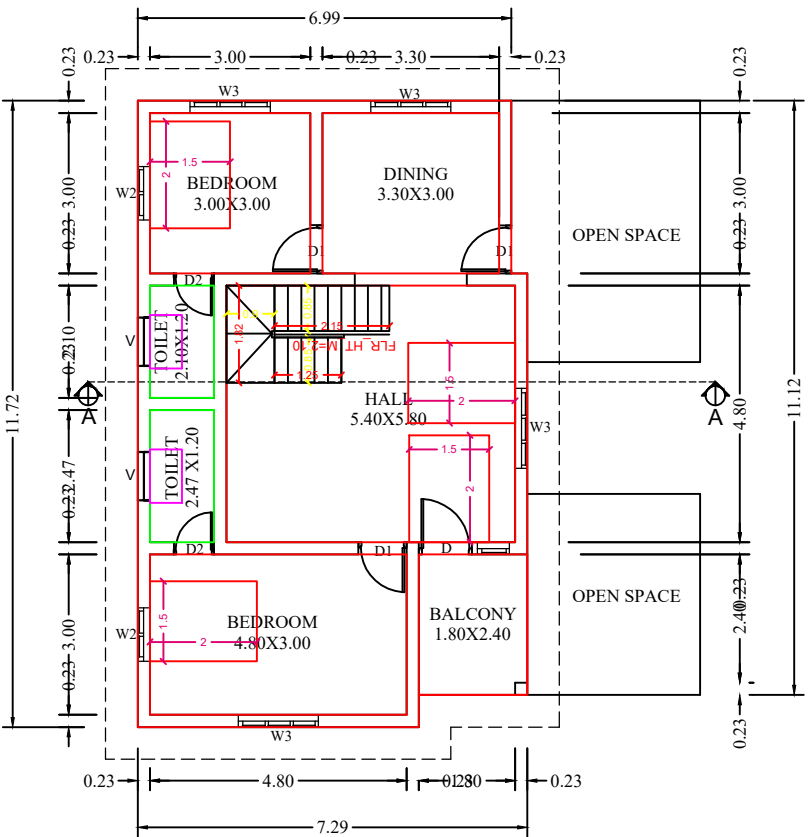
GROUND FLOOR PLAN AREA =83.25 Sq.M (895.77 Sq.ft) SCALE- 1:100
