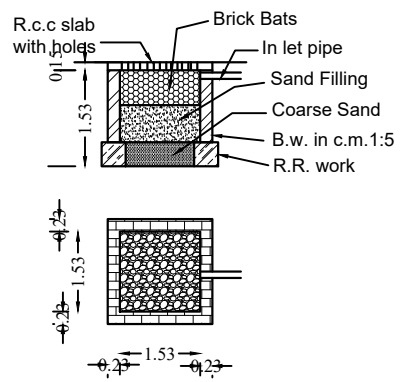
RAIN WATER STORAGE TANK
