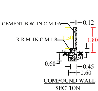
COMPOUND WALL SECTION
