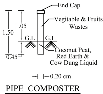
PIPE COMPOSTER
