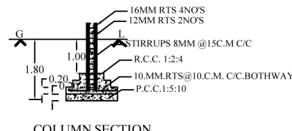
COLUMN SECTION
