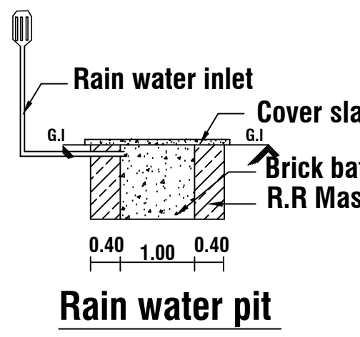
Rain water pit
