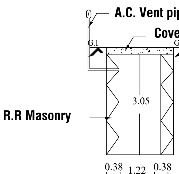
Soakpit section
