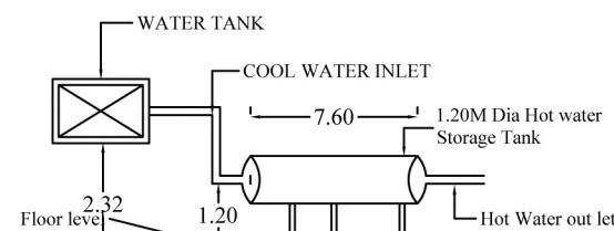
SOLAR WATER HEATING SYSTEM (S.W.H.S.DETAILS)
