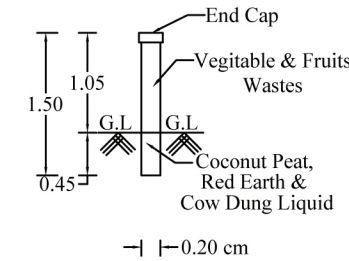
PIPE COMPOSTER
