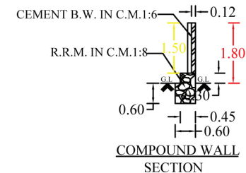
COMPOUND WALL SECTION
