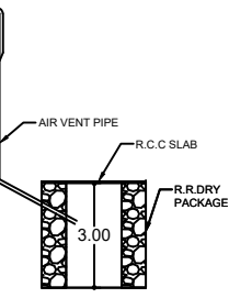
SECTION OF SOAKPIT
