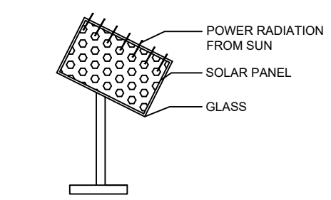
SOLAR SYSTEM
