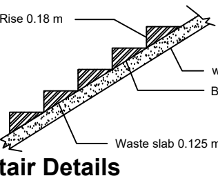
Stair Details
