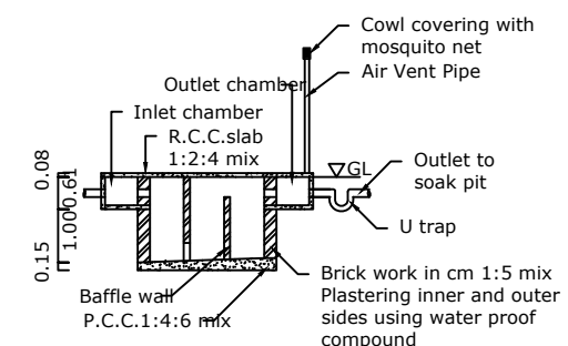
SECTION UV
