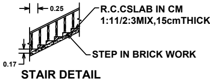
STAIR DETAIL
