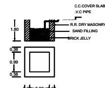
RAINWATER HARVESTING DETAILS
