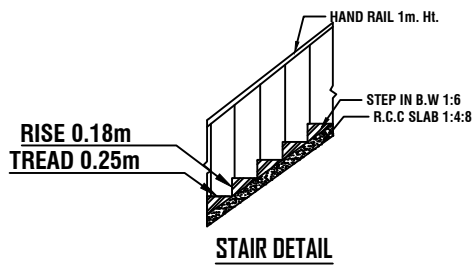
STAIR DETAIL
