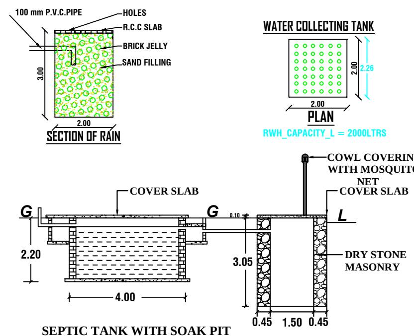
SEPTIC TANK WITH SOAK PIT
