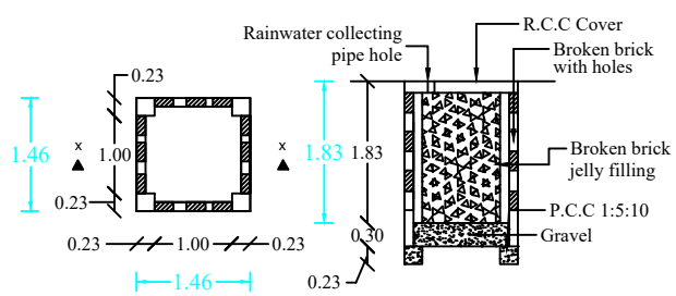
RAIN WATER HARVEST WELL RWH CAPACITY L=6642LTRS
