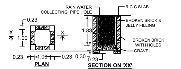
RAIN WATER HARVEST WELL
