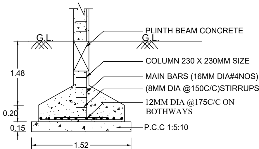
COLUMN FOOTING
