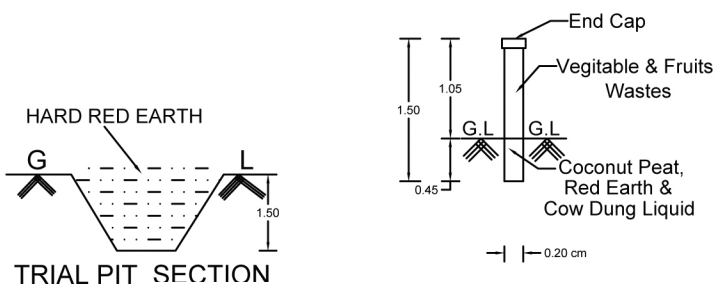
TRIAL PIT SECTION
