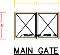
MAIN GATE
