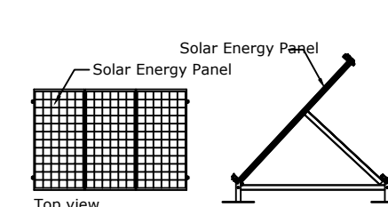
SOLAR POWER SYSTEM
