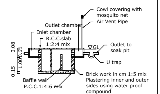
SECTION UV
