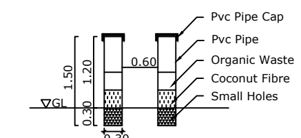
PIPE COMPOST PIT
